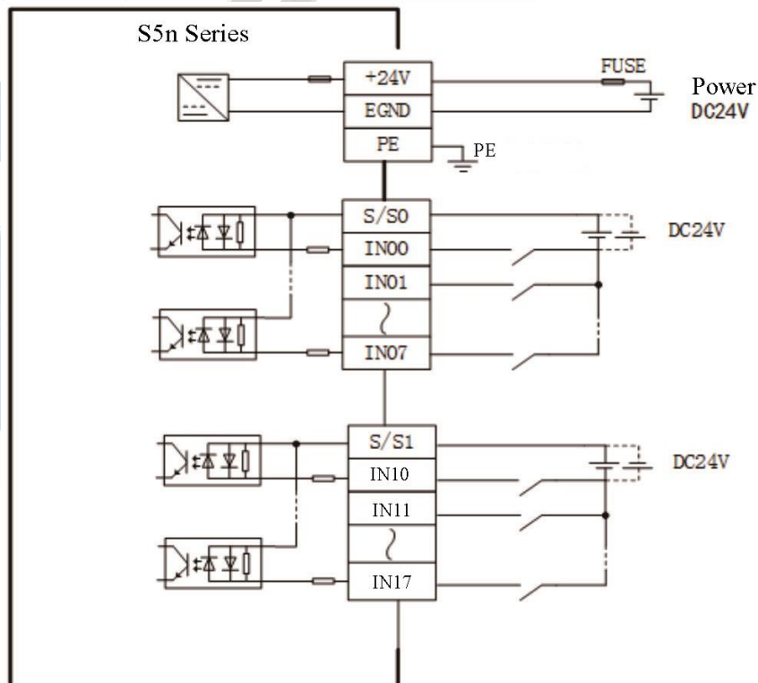
Figure: SC2-C Series Product Input Port Equivalent Circuit
