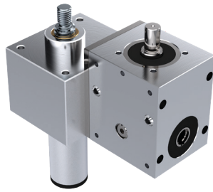
Anschraubposition 90° Mounting position 90°
