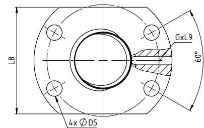
Bohrbild 4 drilling pattern 4 Flansch Form B flange form B nach DIN 69051 according to DIN 69051
