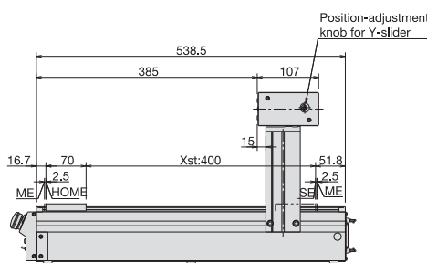
Position-adjustment knob
