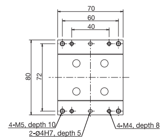
X-axis slider installation hole
