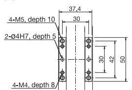
Z-axis slider installation hole
