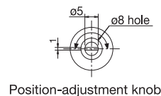
Position-adjustment knob
