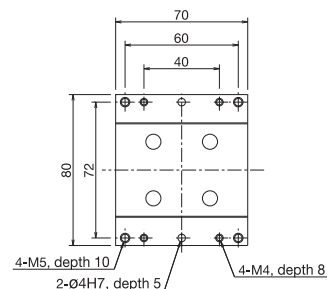
X-axis slider installation hole
