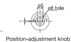
Position-adjustment knob
