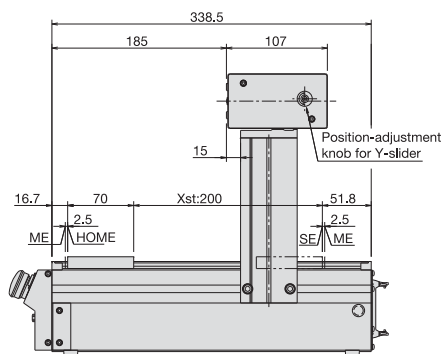
Position-adjustment knob
