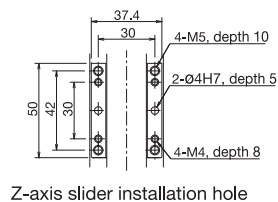
Z-axis slider installation hole
