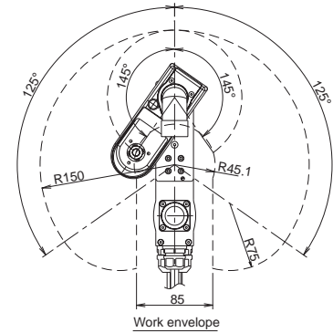
Work envelope
